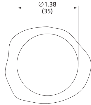
Panel Mounting Cut-Out
